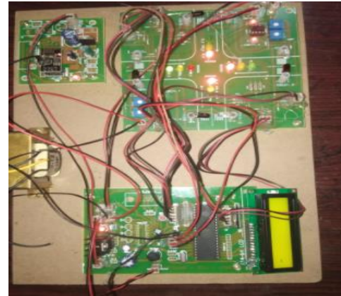
Fig.2. Receiver section side module.
