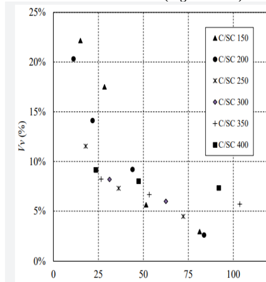
Nominal shear capacity of channel sections (kN)
