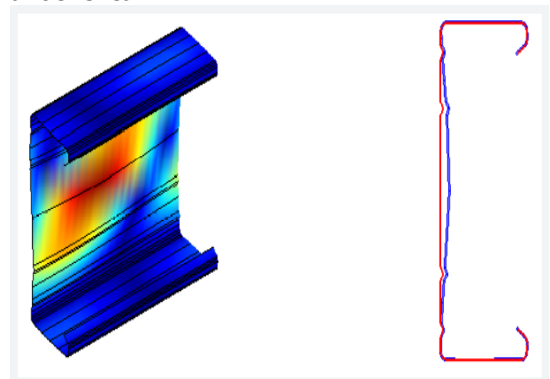
The illustrations of shear buckling mode
