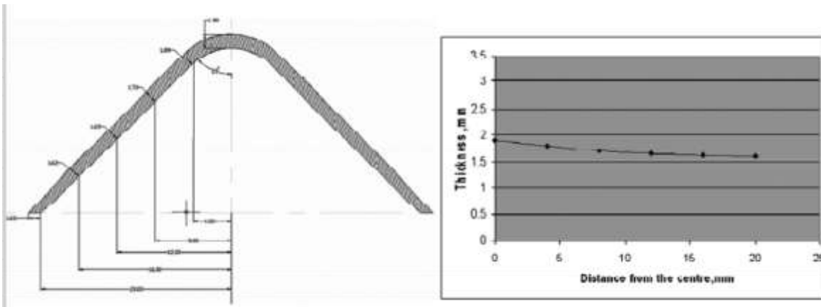
Figure 5: Thickness Variation of the Cone Formed from Centre (Apex) to the Base, for Blank 2
