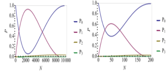
Figure 5. Photon number probabilities for the output field in the strongly coupled line for T = 0.1 . The coupling ratios are a = 0.01 (left) and a = 0.5 (right).
