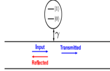
Figure 1. Sketch of the setup considered. A two-level system is coupled to a continuum of left- and right-propagating bosonic modes with coupling strength \gamma .
