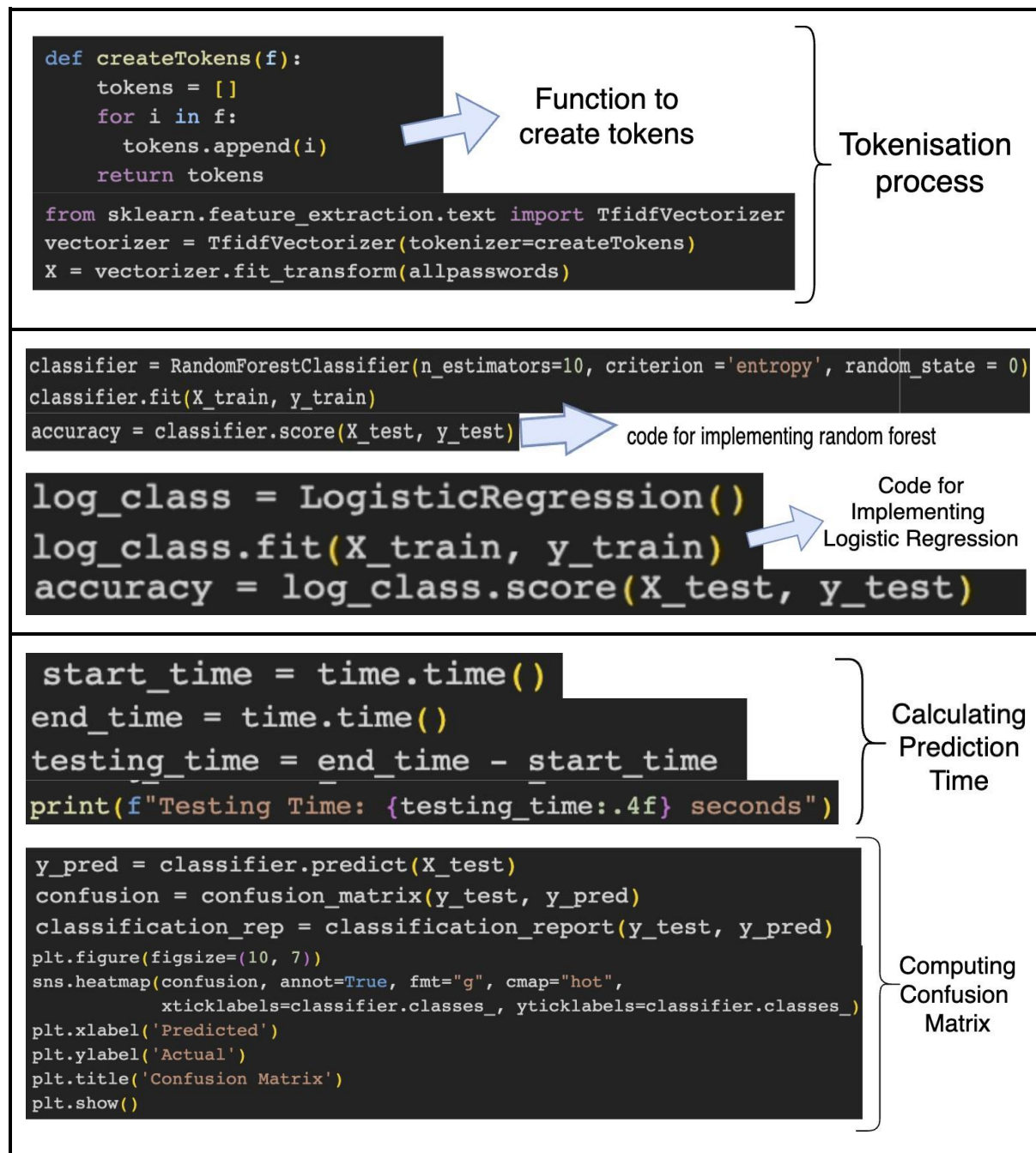
Figure 10: Annotated code corresponding to particular steps in my procedure
