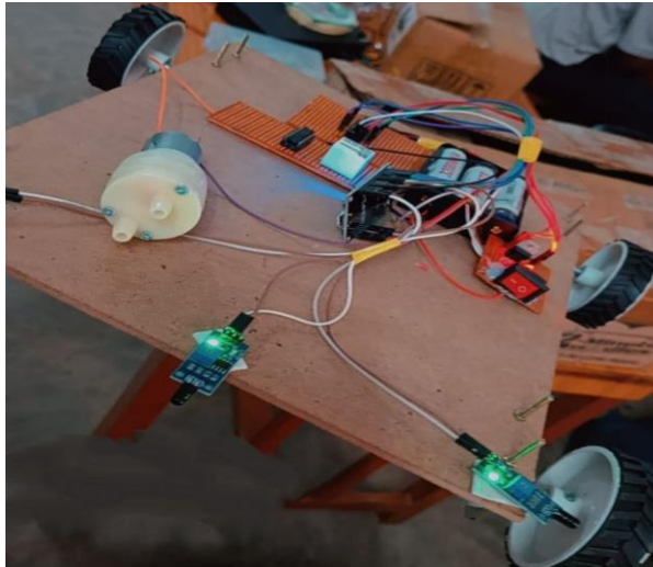
Figure.5 Robotic design
