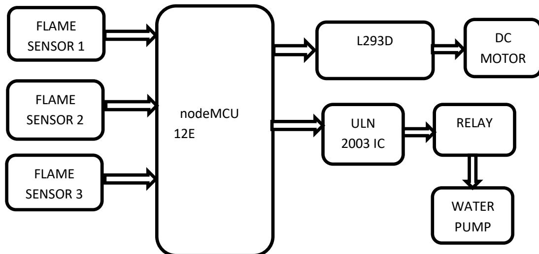
Figure.1 Block diagram
