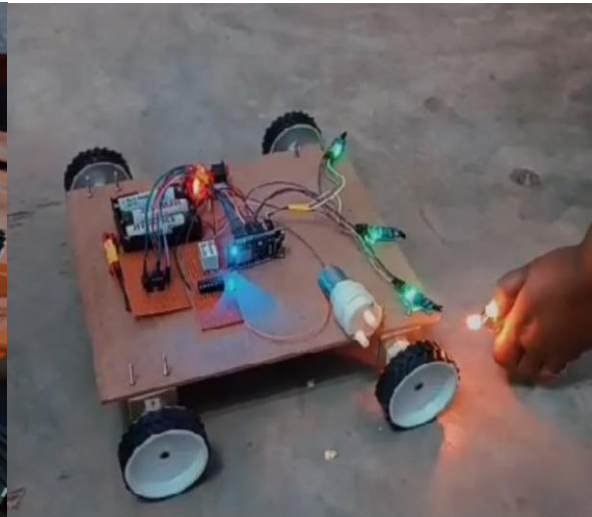
Figure.6 Practical working
