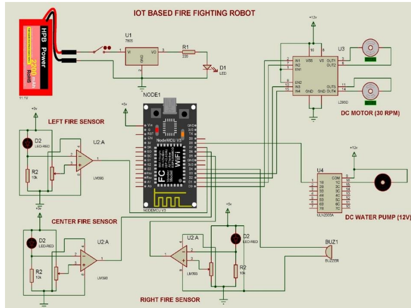
Figure.2 Schematic Diagram
