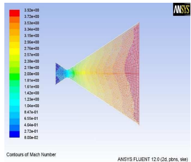
Figure 4.8: Contours of Mach Number
