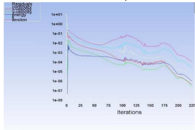
Figure 3.10: Scaled Residuals at Sea Level
