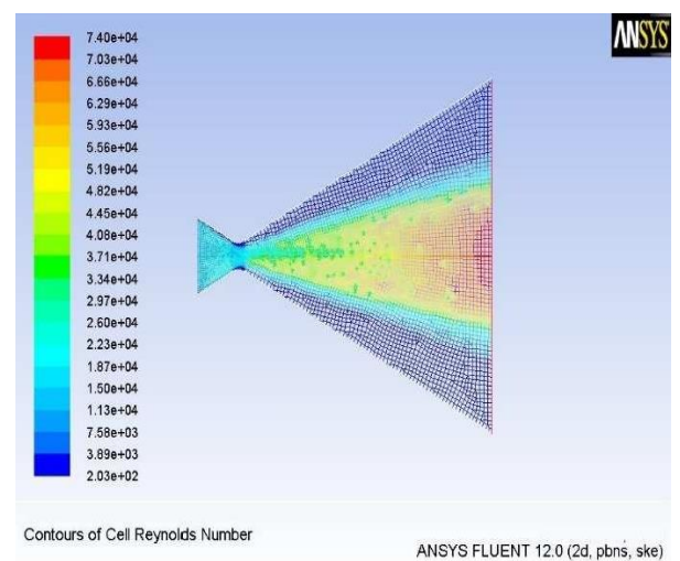
Figure 4.4: Contours of Cell Reynolds Number
