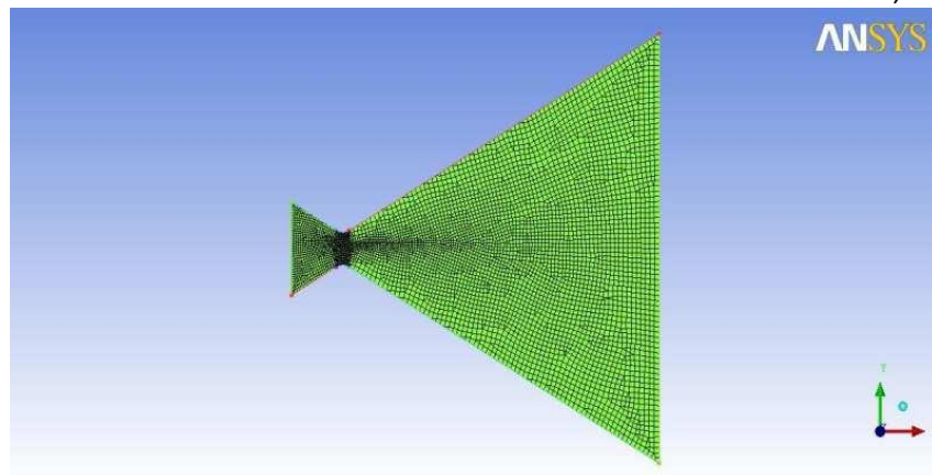
Figure 3.3: Meshed Nozzle
