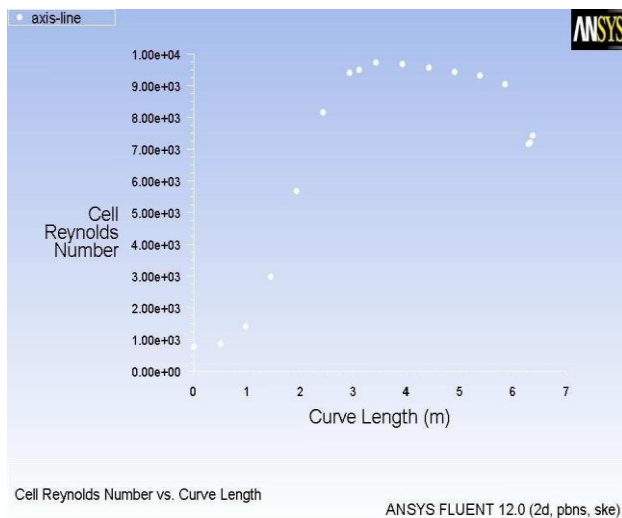
Figure 4.3: Cell Reynolds Number Vs Curved Length
