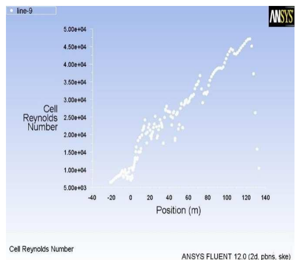
Figure 4.10: Cell Reynolds Number vs Position
