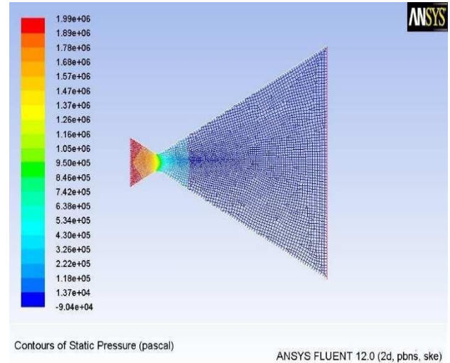
Figure 4.6:: Contours of Static Pressure
