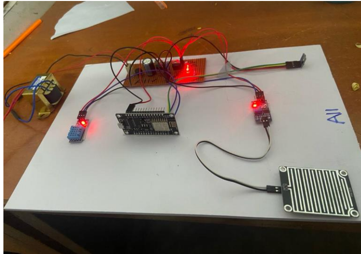
Figure.3 working kit
