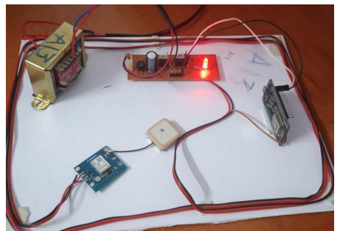
Figure.3 Working kit
