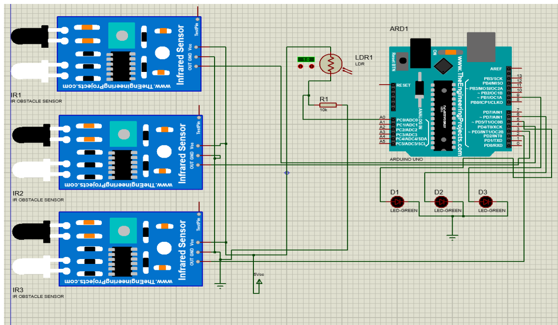
Figure.2 Schematic Diagram
