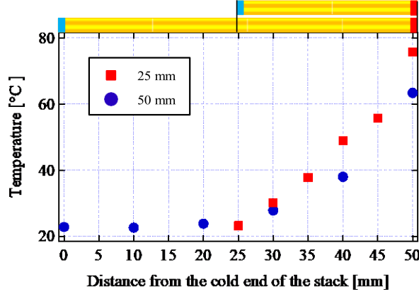
Figure 3. Temperature distribution in the stack immediately after starting oscillation
