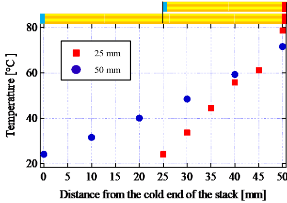
Figure 4. Temperature distribution in the stack at steady condition
