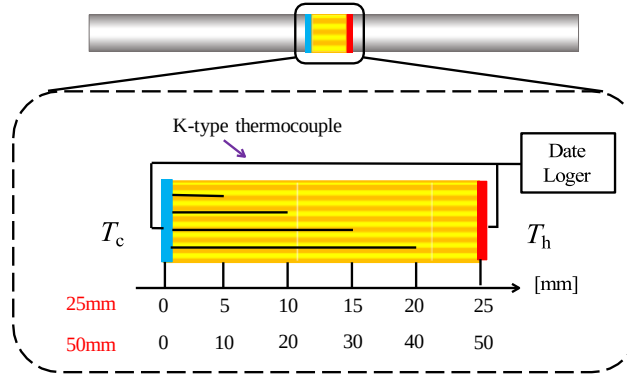
Figure 2. Temperature measurement system
