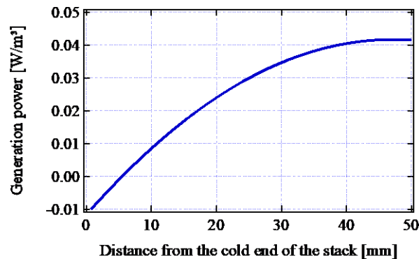
Figure 5. Generated power distribution immediately after starting oscillation
