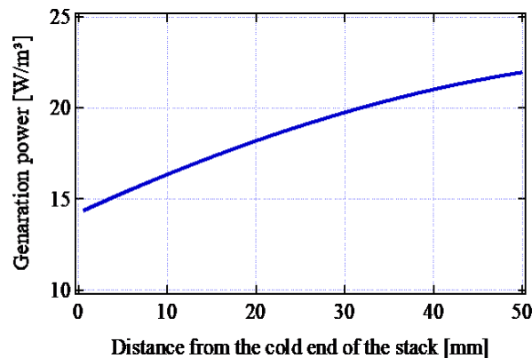
Figure 6. Generated power distribution at steady condition
