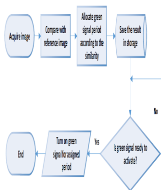
1.1 Proposed time allocation algorithm for autonomous traffic control System
