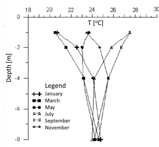
Figure 1. Temperature evolution in subsurface soil layer at different times in Hanoi [1].
