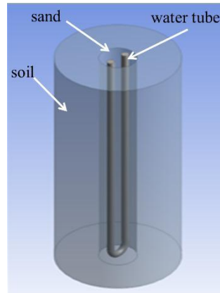
Figure 3. The geometry of underground heat exchanger.
