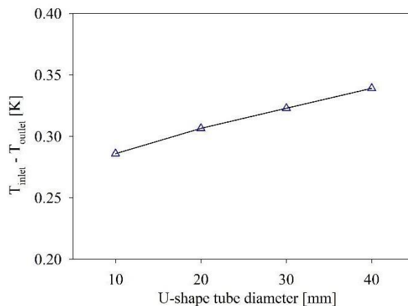
Figure 7. Influence of U-shape tube diameter on the temperature difference between inlet and outlet water. The connecting line is aid of eye.
