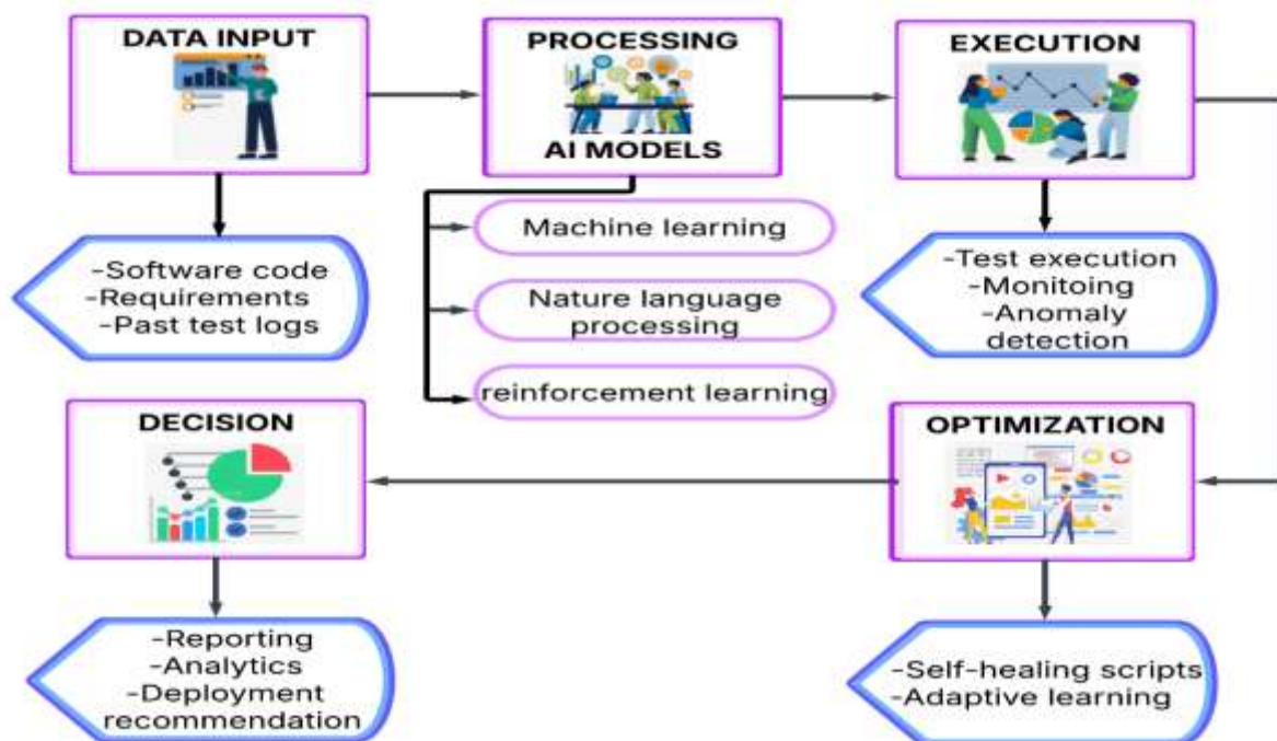
Figure 1 AI-Driven Automation Framework for Software Testing and Optimization
