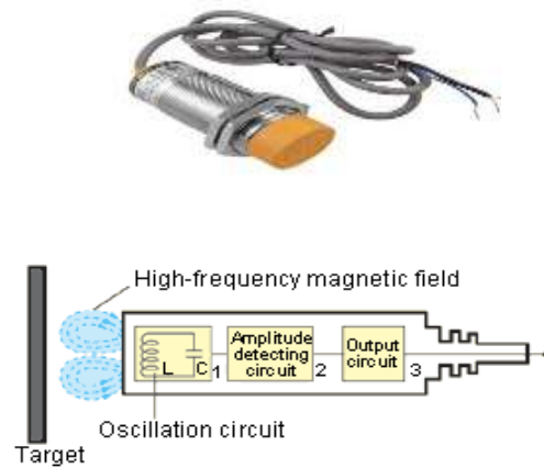
FIG 3.22:Proximity Sensor
