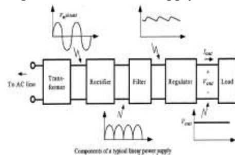
FIG 3.3:Block Diagram of Power Supply
