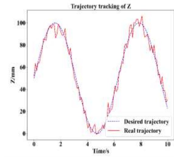
Figure 2: Z-Axis Trajectory Tracking Performance
