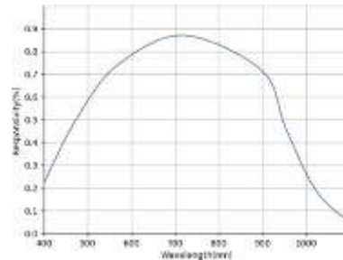
Fig.2. CMOS image sensor's photosensitive range.
