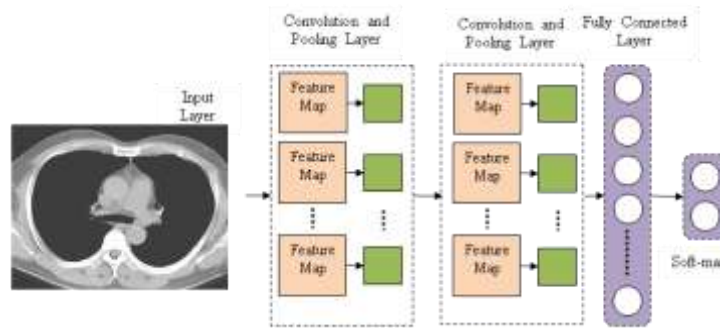
Fig. 1 The architecture of Covid-19 Disease prediction Model
