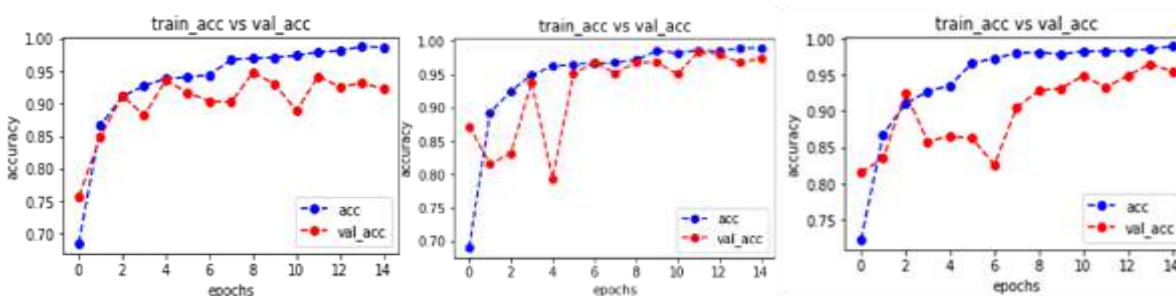
Fig. 10 Classification accuracy for Covid-19 with 10-Fold validation
