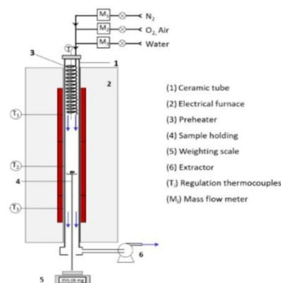
Figure 1. MTG reactor
