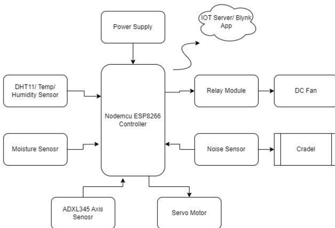
Figure1: Block Diagram of Smart Baby Maintenance and Monitoring System
