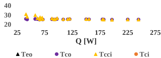
Figure 7. Temperatures at different locations vs heat load using water as the working fluid, using the new design evaporator
