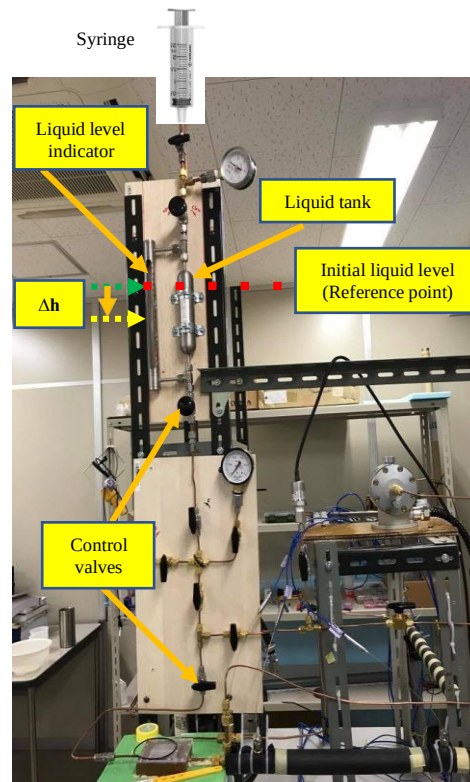
Figure 5. Photograph of experimental charging system
