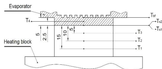
Figure 3. Temperature measurement inside heating block
