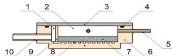
Figure 1. Schematic diagram of the previous evaporator 1: vapor collector; 2: compensation chamber; 3: poly carbonate lid; 4: O-ring; 5: charging pipe; 6: copper evaporator body; 7: wick; 8: vapor grooves; 9: copper plate; 10: vapor pipe.
