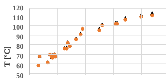
Figure 6. Temperatures T_{s1} varied with heat load, compared with the previous and new design evaporators
