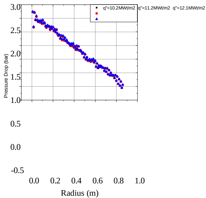
Figure 8. Pressure drop of coolant in a heat channel
