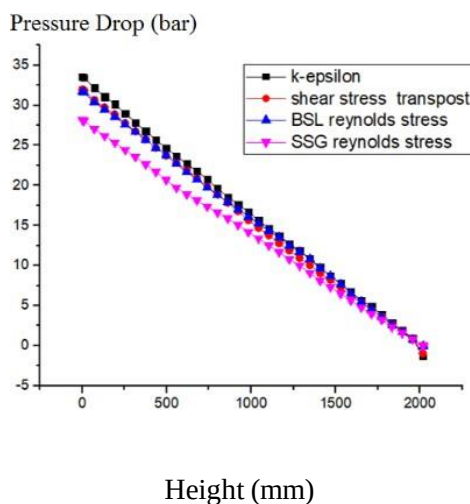
Figure 12. Pressure drop of coolant in a heat channel
