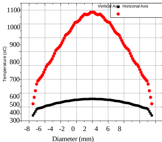
Figure 14. Temperature distribution of a fuel element
