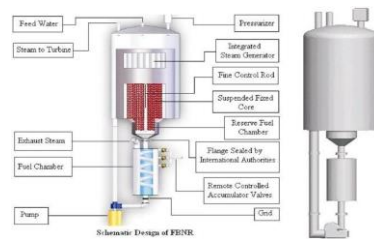
Figure1. Schematic design of FBNR.
