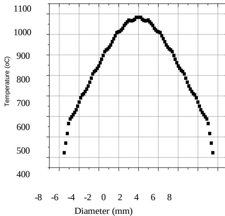
Figure 9. Temperature distribution of a fuel element
