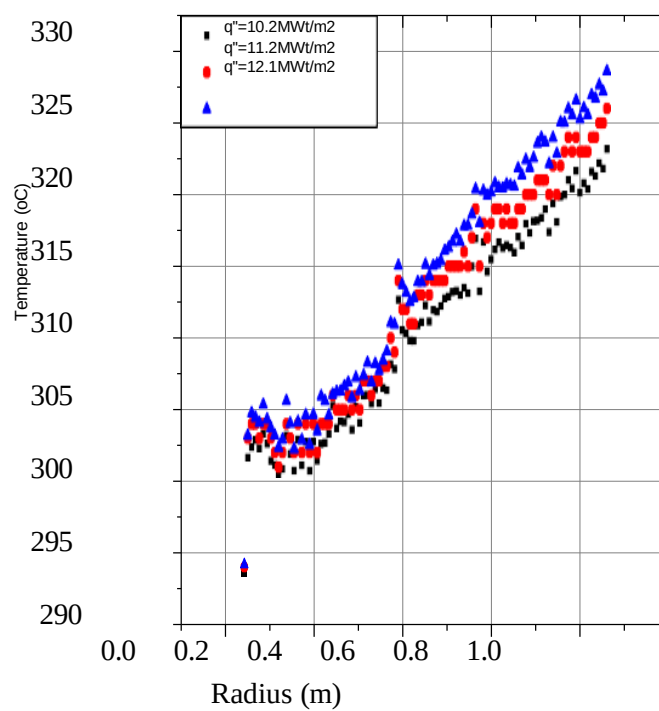
Figure 6. Temperature of coolant in a heat channel
