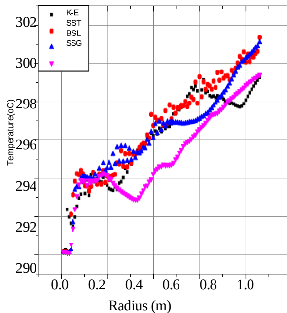
Figure 3. Temperature of coolant in a heat channel
