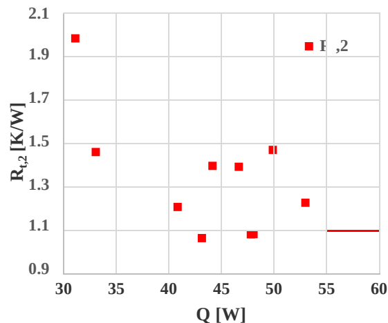
Figure 10. Total thermal resistance of the ethanol LHP with the new design evaporator
