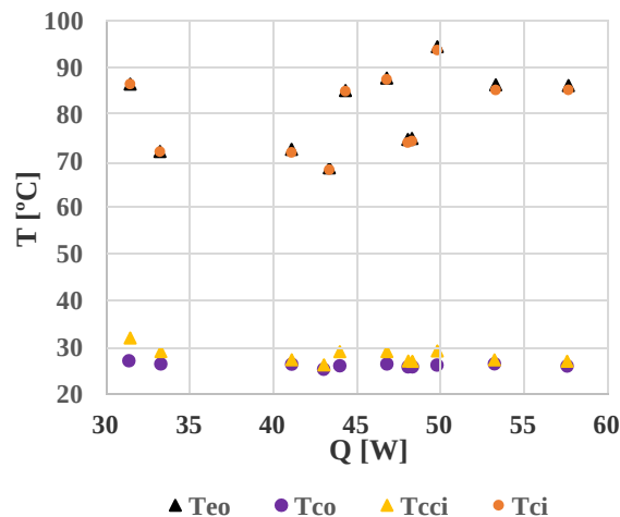
Figure 8. Temperatures at different locations vs heat load using ethanol as working fluid, using the new design evaporator
