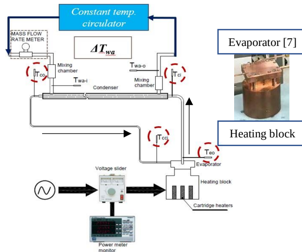
Figure 2. Schematic diagram of experimental setup
