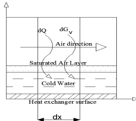
Figure 1. Heat and mass transfer mechanism of moist air outside the tube.
