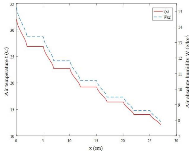
Figure 4. Variation of absolute humidity and temperature of moist air along the coil for the 1 st case.
