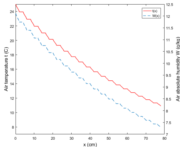
Figure 5. Variation of absolute humidity and temperature of moist air along the coil for the 2 nd case.
