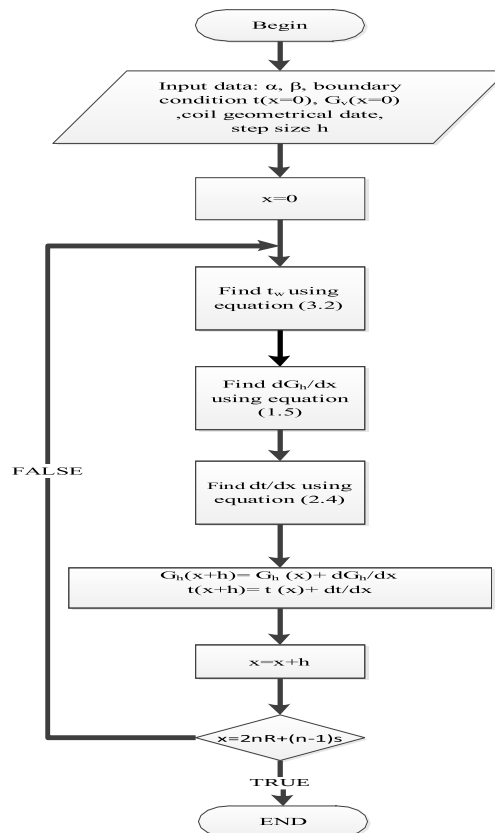
Figure 3. Flowchart of the simulation program
