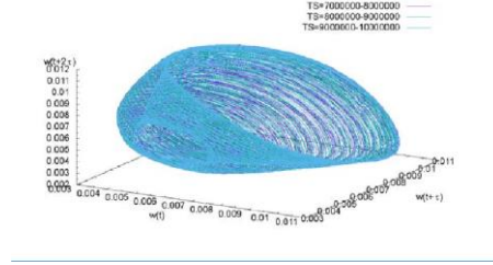
Figure 10. \Gamma=7.6 and Re=1080 (Number of time steps = 2 million to 5 milli
