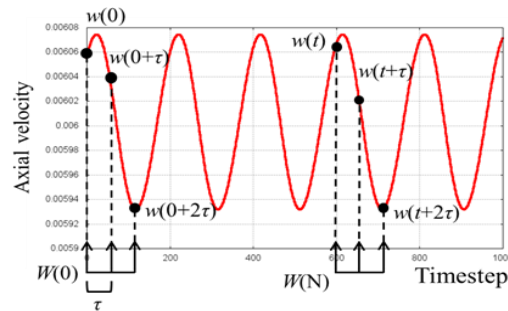
Figure 3. Embedding of Functions W(w(t), w(t+\tau), \text{ and } w(t+2\tau)) into Three-dimensional Coordinate System
