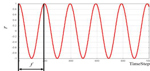
Figure 5. Autocorrelation Function ( r(t) ) of Axial Velocity ( w(t) )
