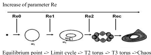
Figure 2. Ruelle-Takens-Newhouse Scenario
