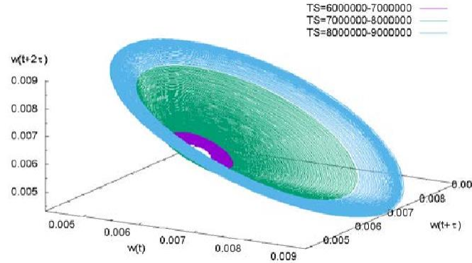
Figure 13. \Gamma=7.7 and Re=1060 (Number of time steps = 6 million to 9 million)
