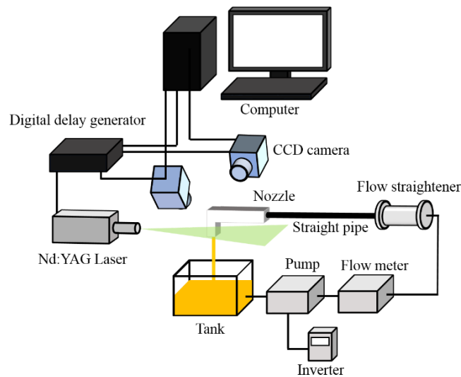
Figure 4. Experimental apparatus for stereo PIV experiment
