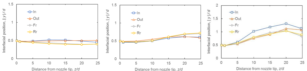
Figure 6. Interfacial position of each sides at Re=1500 (left), 2000 (center), 2500 (right)
