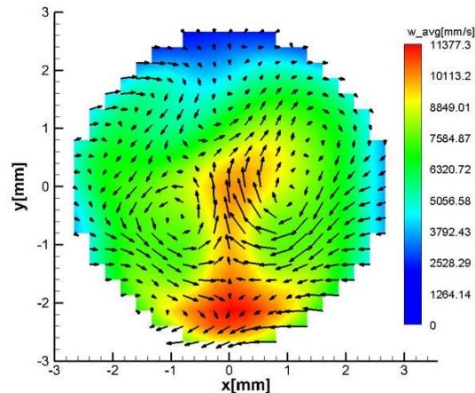
(c) Flow distribution at L/d=5 at Re=2500
