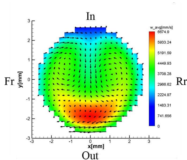
(a) Flow distribution at L/d=5 at Re=1500
