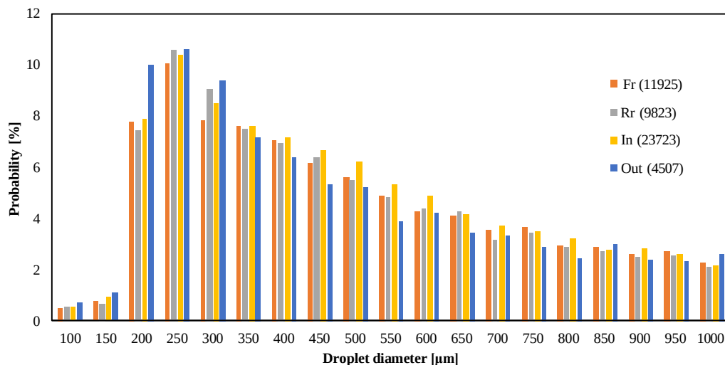
(a) The droplet diameter distribution at Re=2500
