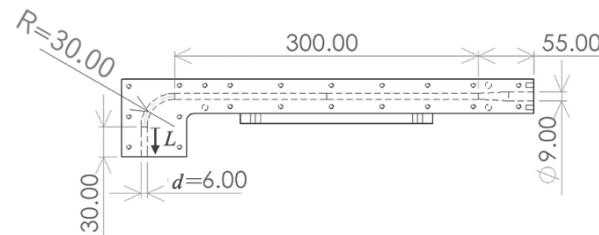
Figure 1. The size of nozzle for visualization experiment
