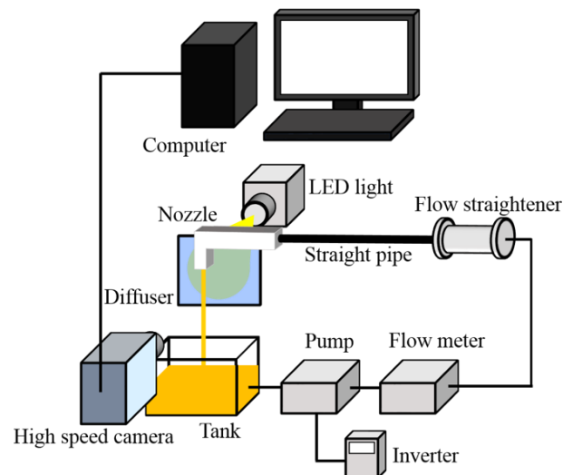
Figure 3. Experimental apparatus for visualization experiment
