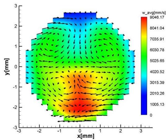
(b) Flow distribution at L/d=5 at Re=2000
