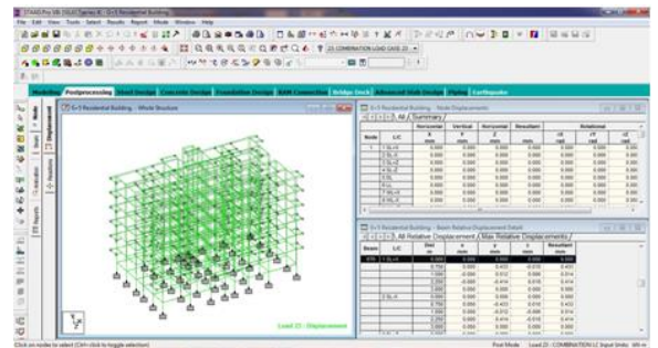
Fig.3.5. Post processing mode in STAAD.Pro
