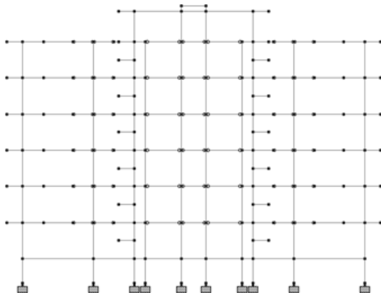
Fig.3.2. Elevation of the G+5 storey building.
