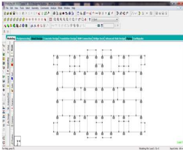
Fig.3.1. Plan of the G+5 storey building.
