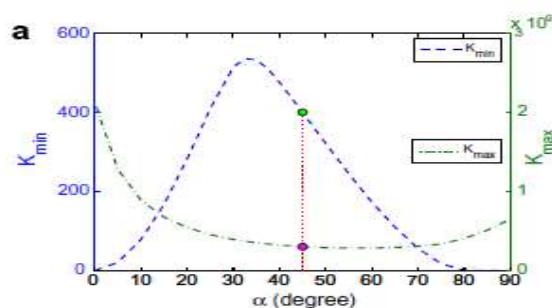
Fig. 7. The distribution for (a) minimum and (b) maximum stiffness in a plane of z = 0.242 m.
