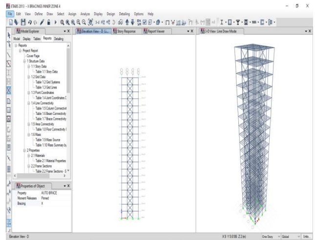
Figure 3.6 Elevation and 3D view of the building with X bracings at center bay
