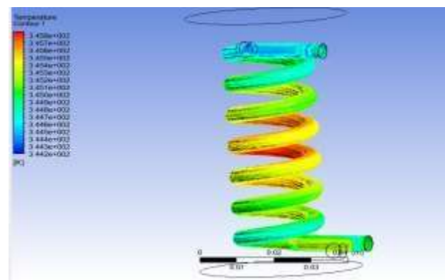
Fig:10 Temperature contour (R744)
