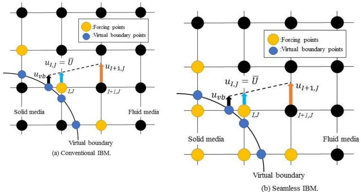
Figure 1. Grid points added forcing term
