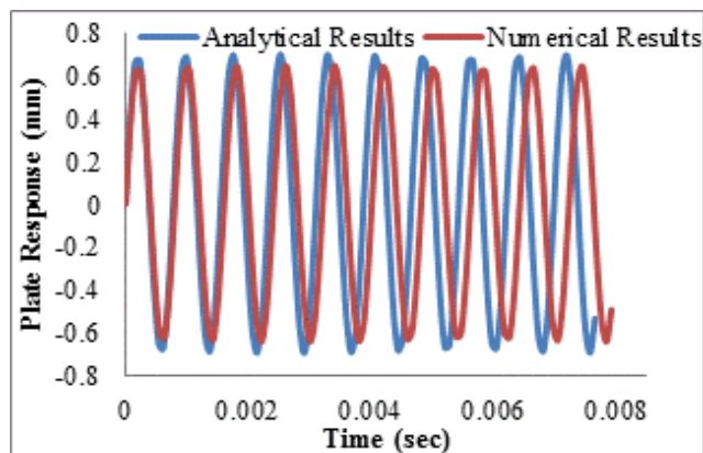
Figure 27. Comparison Between Analytical and Numerical Plate Response Results with T0 Temperature Effect of 6061 Aluminum Alloy
