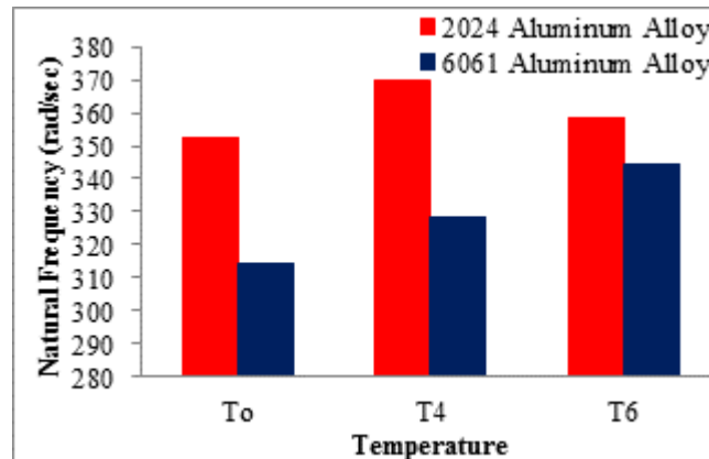
Figure 23. Natural Frequency for Various Aluminum Alloy Cantilever Supported Plate, with Different Temperature Effect
