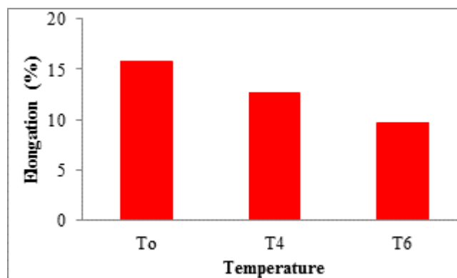
Figure 15. Elongation for 2024 Aluminum Alloy with Various Heat Treatment Effect
