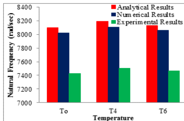
Figure 18. Comparison of Natural Frequency for Simply Supported Plate of 2024 Aluminum Alloy, Evaluated by Different Techniques
