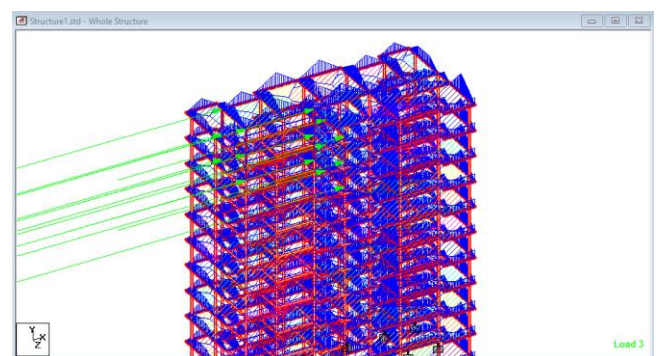
Fig.3.1. Self-weight Z1.
