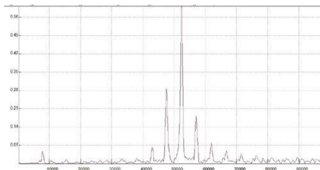
b. Vibration Response Signal (mv) with Frequency (Hz) Relationship
