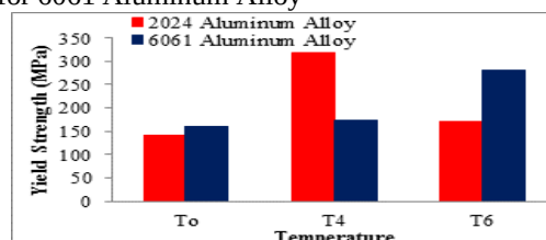
Figure 7. Yield Strength for 6061 Aluminum Alloy
