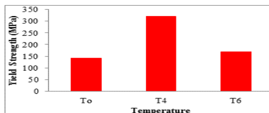
Figure 6. Yield Strength for 2024 Aluminum Alloy with Various Heat Treatment Effect
