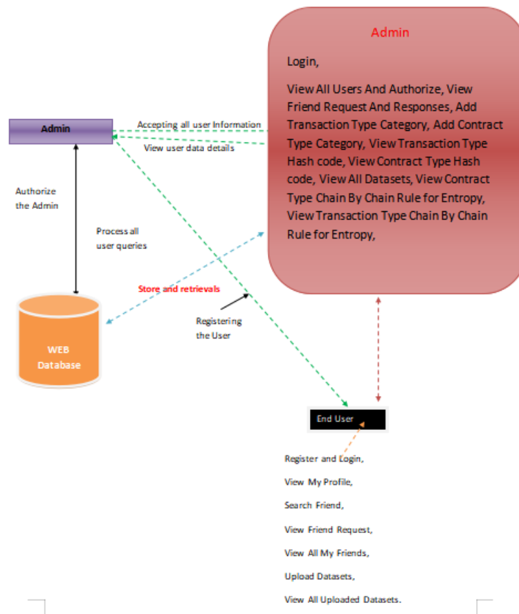
Fig:Architecture diagram
